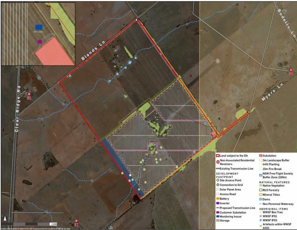
Layout of West Wyalong Solar Farm
